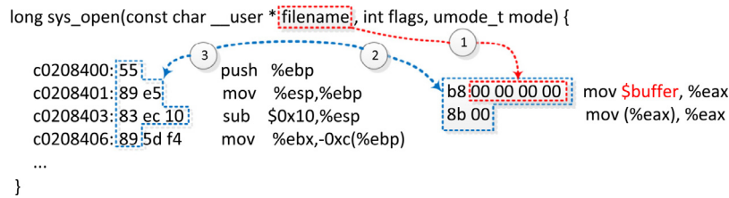
Fig. 2 – Enforced mapping on unmapped buffer. (1) Load filename’s memory address into $buffer. (2) Replace the first 7-byte instructions of the function body with mov $buffer,%eax;mov (%eax),%eax . (3) Rewrite the original instructions back and re-execute them.
